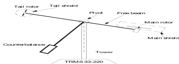
Fig 1. The TRMS
